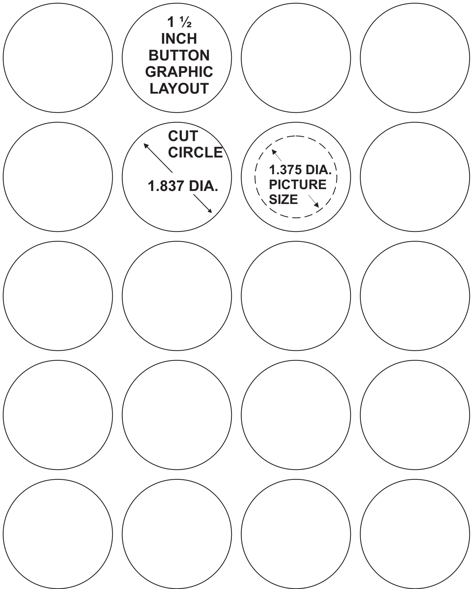
1 1/2 INCH BUTTON GRAPHIC LAYOUT for the Manual or Electric Button Maker Machine LARGE CIRCLE IS CUT LINE. SMALL DASHED LINE IS RECOMMENDED MAXIMUM PICTURE SIZE.
